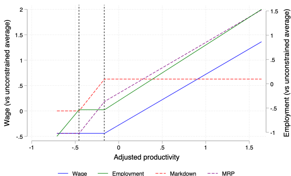
Figure 2: Model simulation
